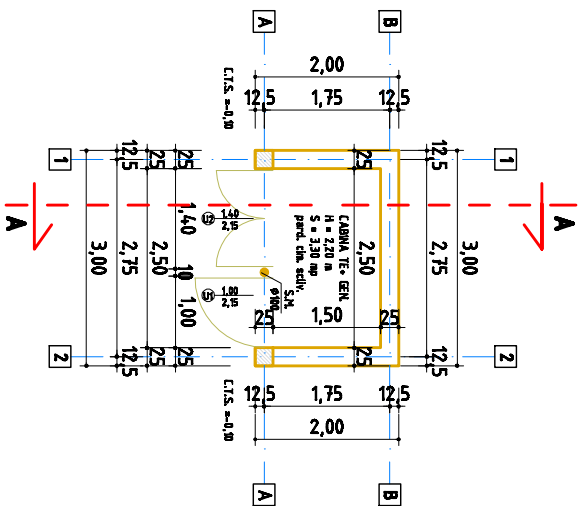
PLAN CABINA TE + GENERATOR
