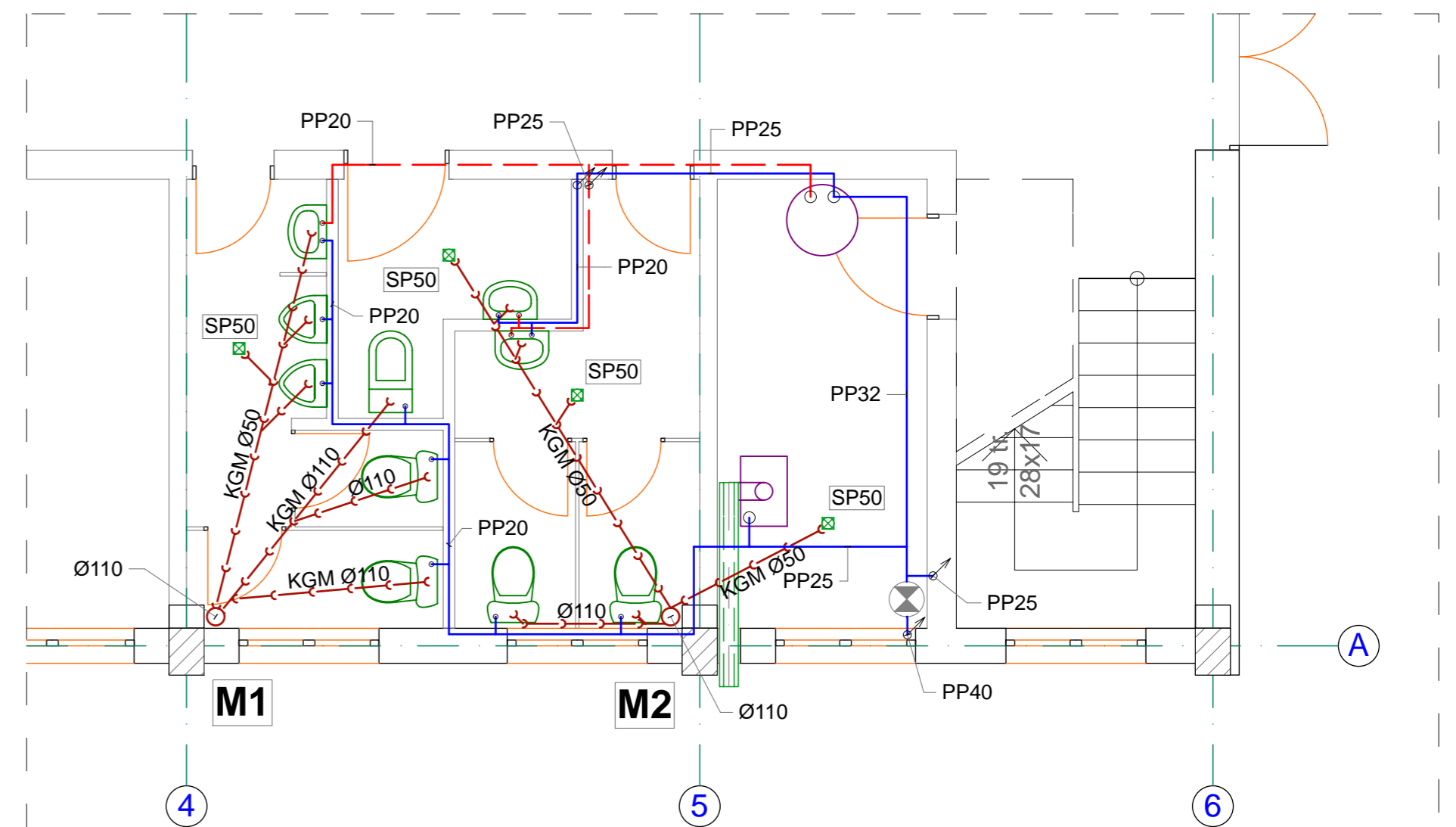
PLAN PARTER
