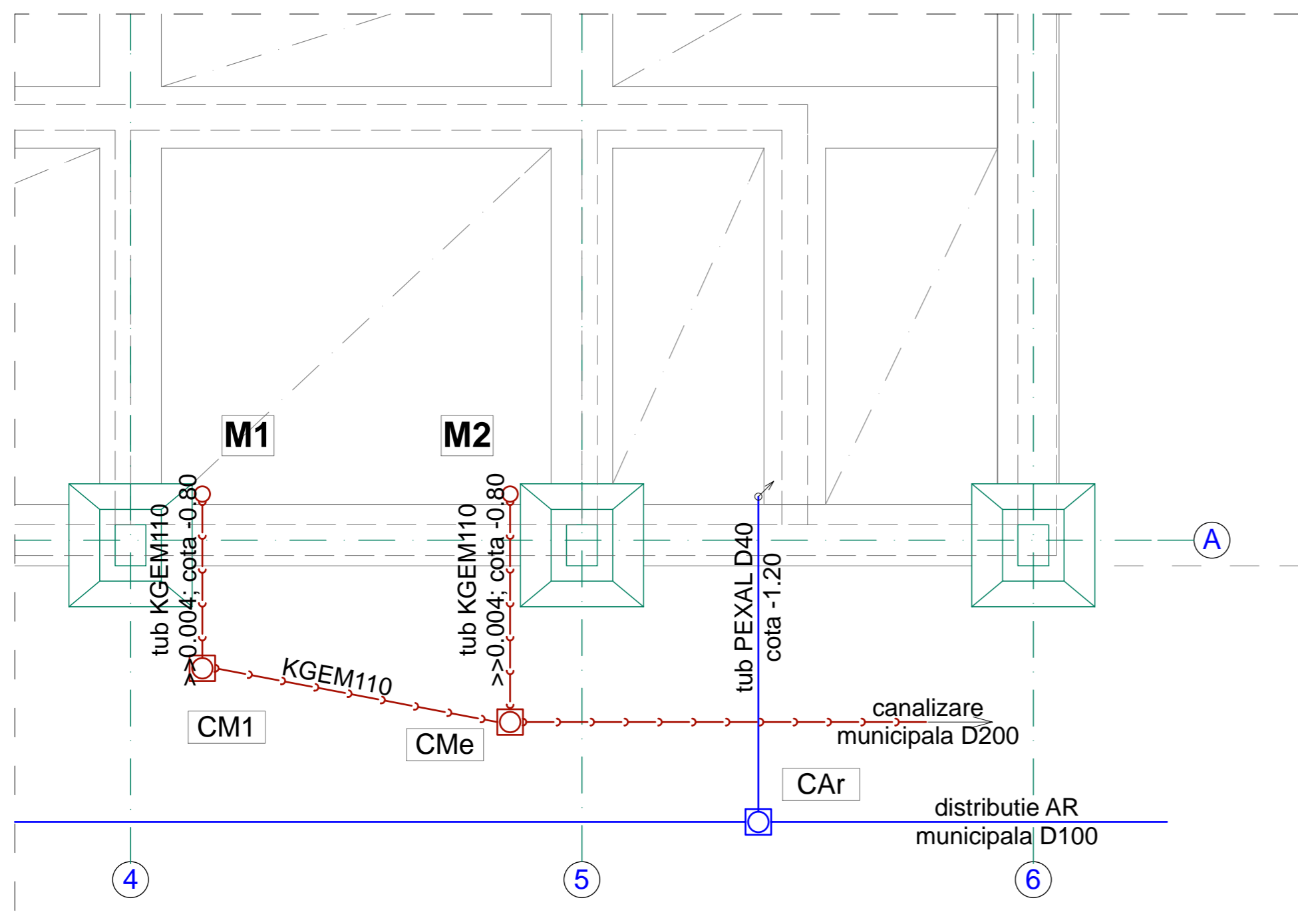
PLAN RACORD - cota -1.20
