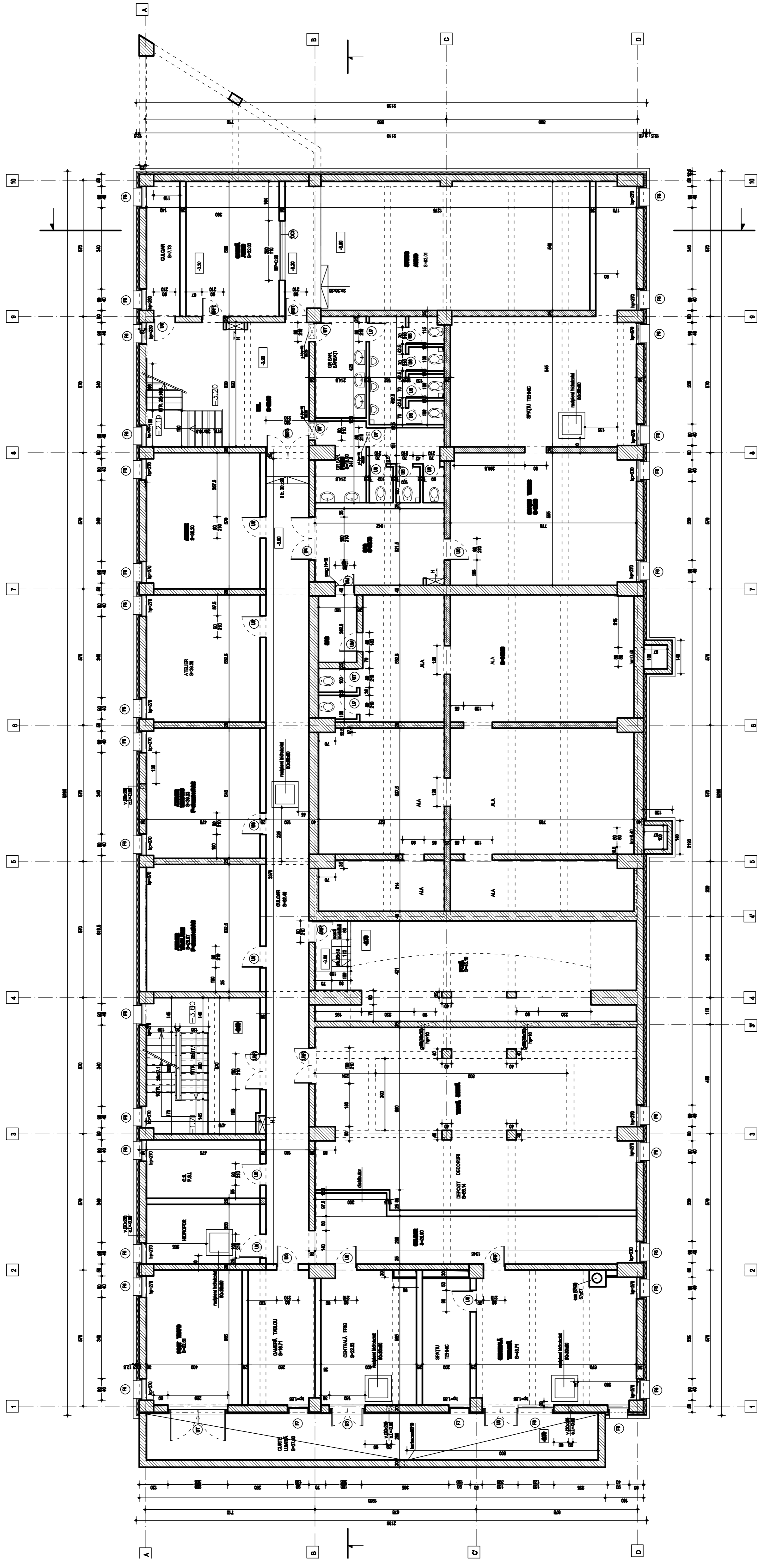
PLAN SUBSOL
